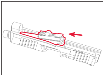
INSTALL BARREL
