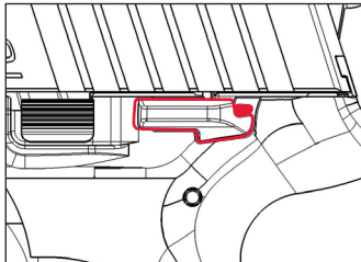
SAFETY DISENGAGED
