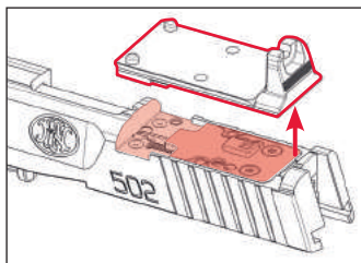
FN OPTICS MOUNTING SYSTEM
