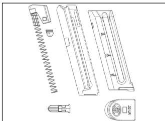
MAGAZINE COMPONENTS - 15 RD
