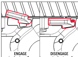
MANUAL SAFETY
