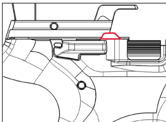
TRIGGER DISCONNECT
